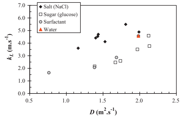
Fig. 7. Liquid-side mass transfer coefficients versus oxygen diffusion coefficients ( T = 20^\circ C ).
