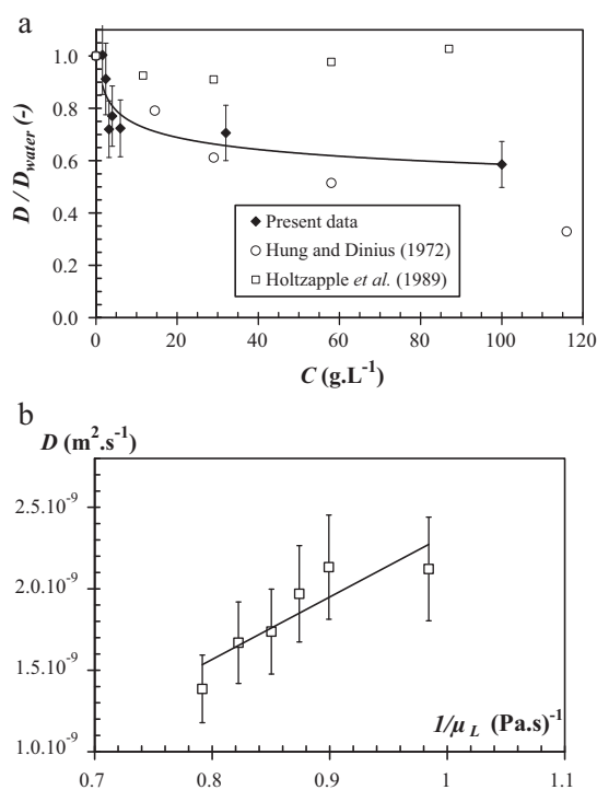
Fig. 4. (a) Comparison between the oxygen diffusion coefficients in aqueous solutions of salt measured and the ones reported in the literature. (b) Oxygen diffusion coefficient versus inverse of viscosity for aqueous solutions of glucose.
