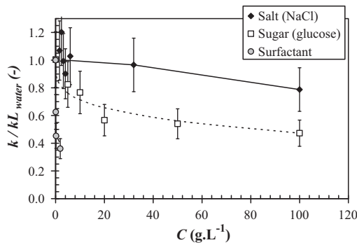
Fig. 6. Ratio between liquid-side mass transfer coefficients in synthetic liquid media and in clean water versus the concentration of the compound introduced (salt, sugar or surfactant) ( T = 20^\circ C ).
